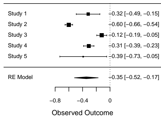
Figure 7: Plot of PD and AL with their forest plots
